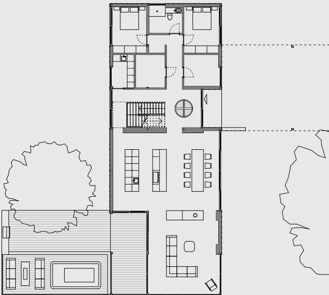
Left First- and ground-floor plans; section.
