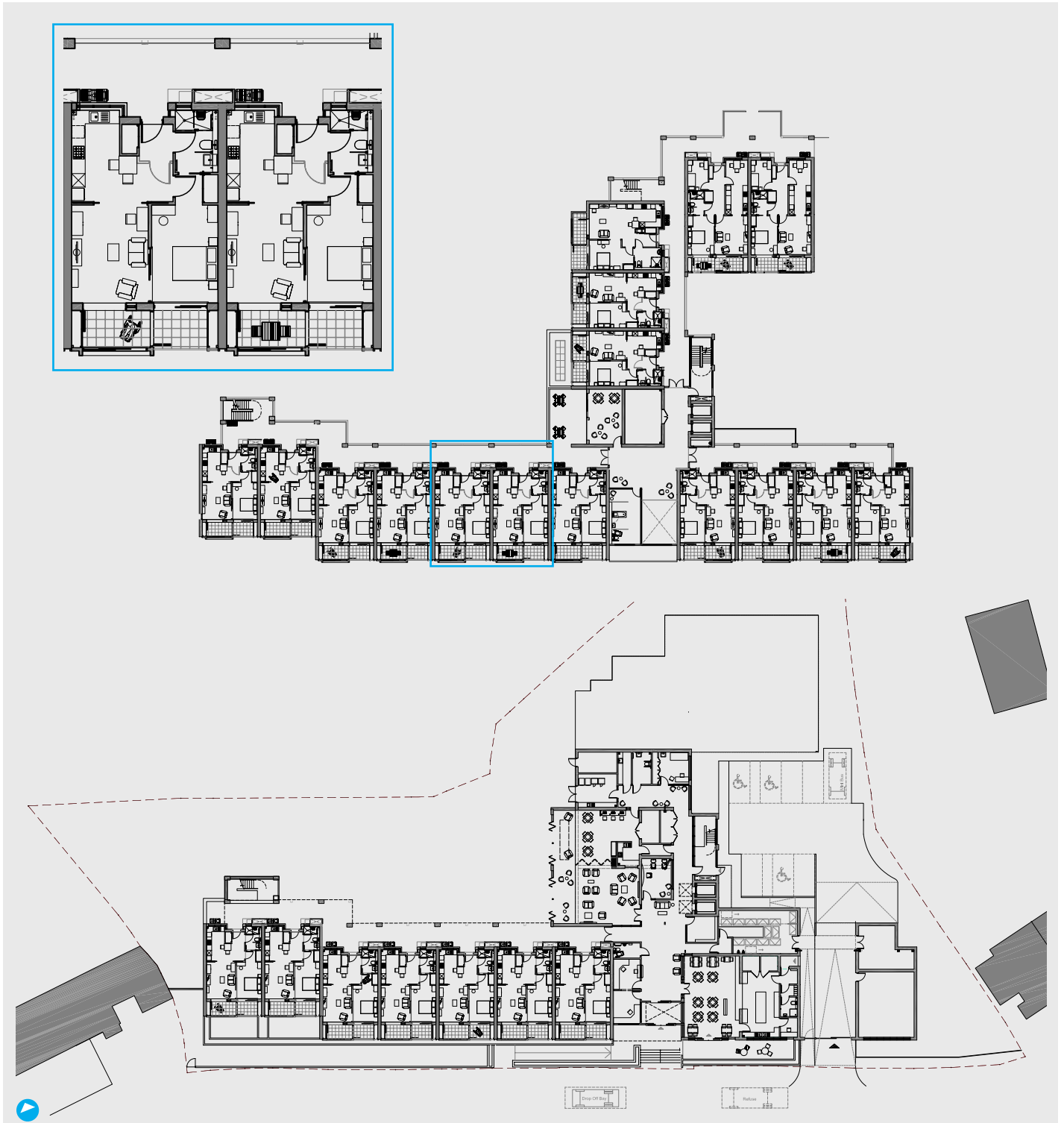
Above Ground and upper floor plans; typical flat plan. Apartments range from 54 square metres for typical one-beds to 78 square metres for typical two-beds.
